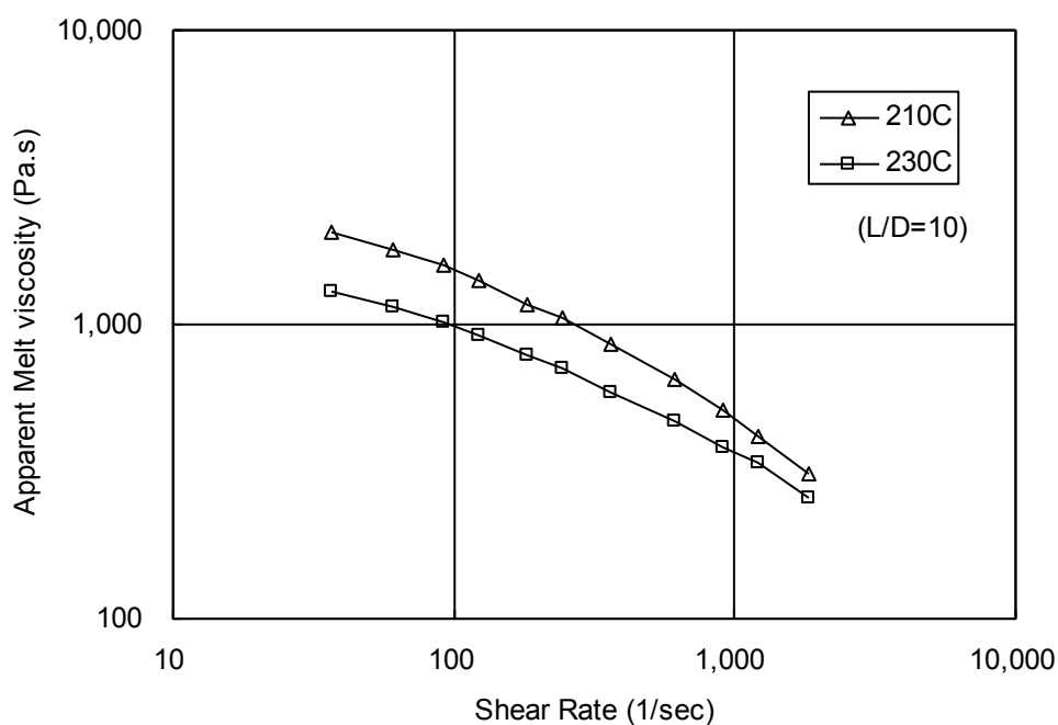
Fig. 1 Melt Viscosity of SoarnOL™ TF2905B
