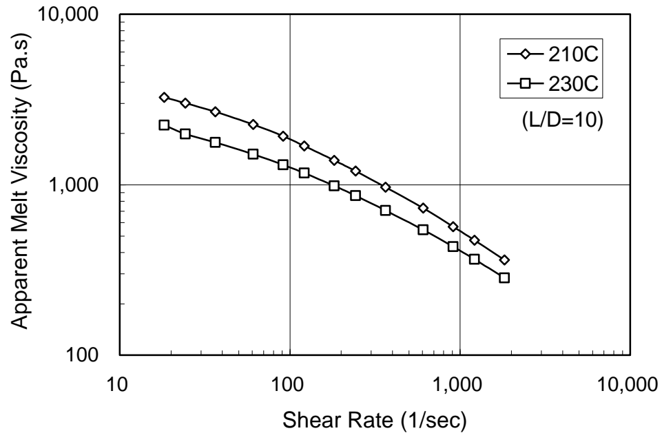
Fig. 1 Melt Viscosity of Soarnol™ DT2904R
