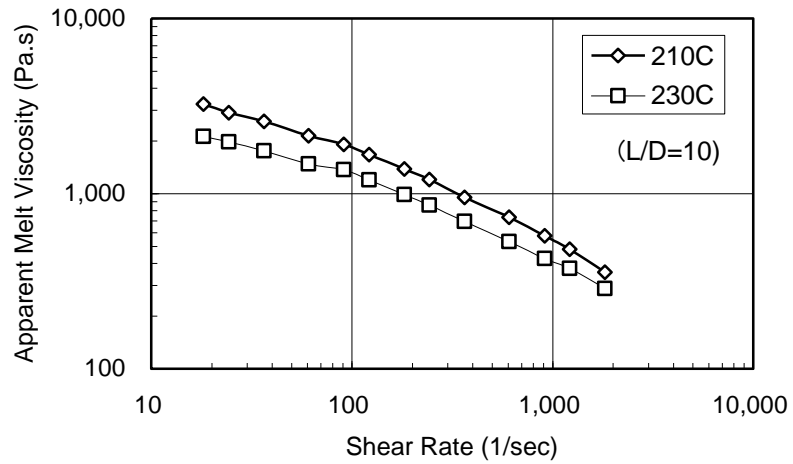
Fig. 1 Melt Viscosity of Soarnol™ DC3203RB
