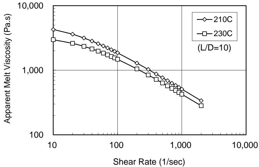
Fig. 1 Melt Viscosity of Soarnol™ DC3203FB
