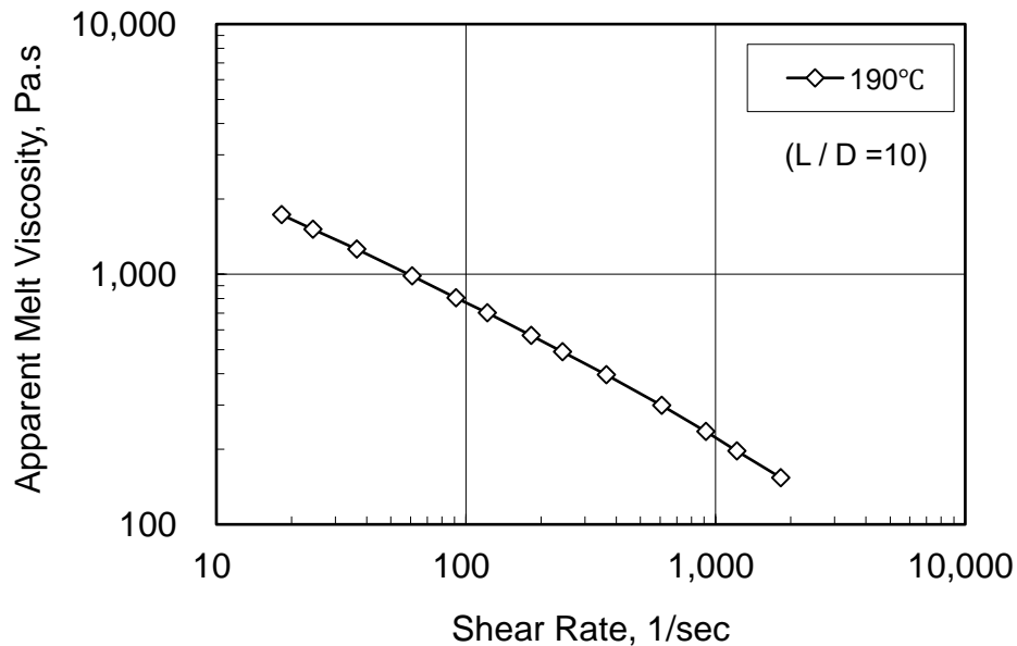
Fig. 1 Melt Viscosity of Soaresin™ RG100
