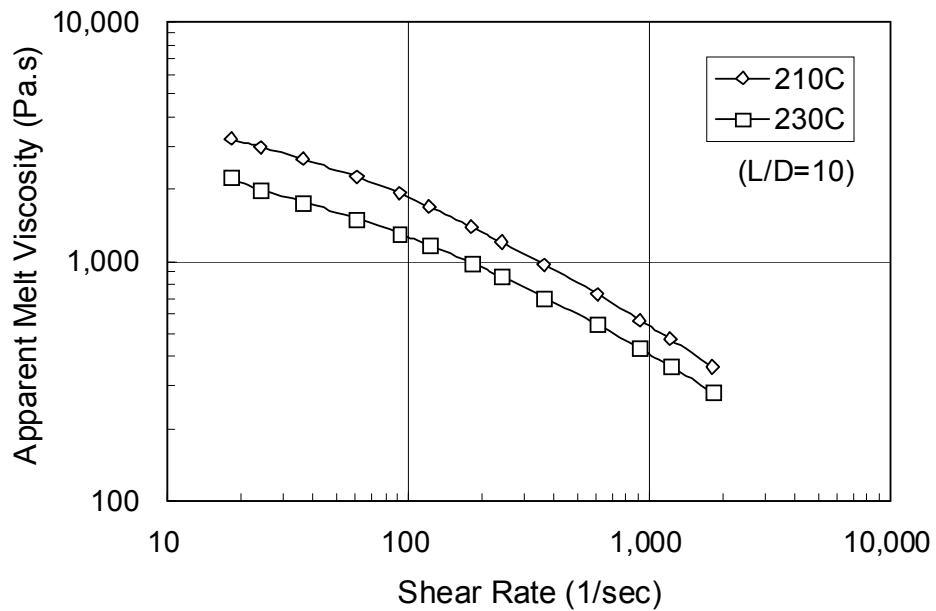
Fig. 1 Melt Viscosity of Soamol™ DT2904R
