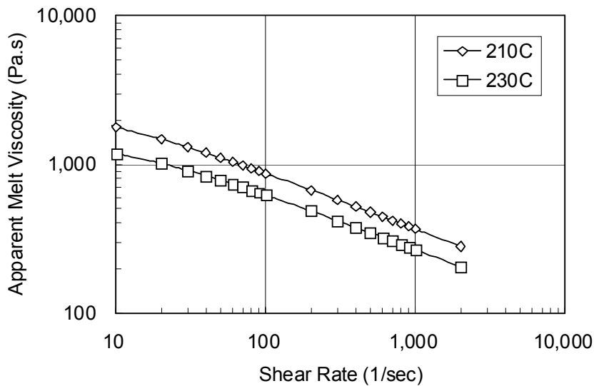
Fig. 1 Melt Viscosity of Soarnol™ DC3212B
